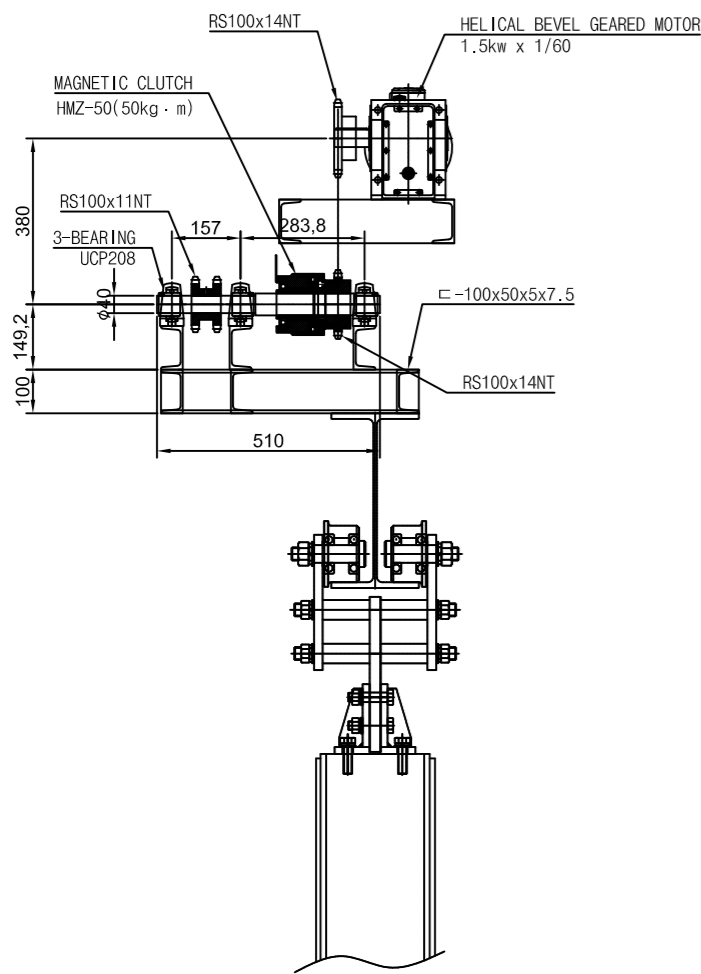
SECTION A-A SCALE=5/56
