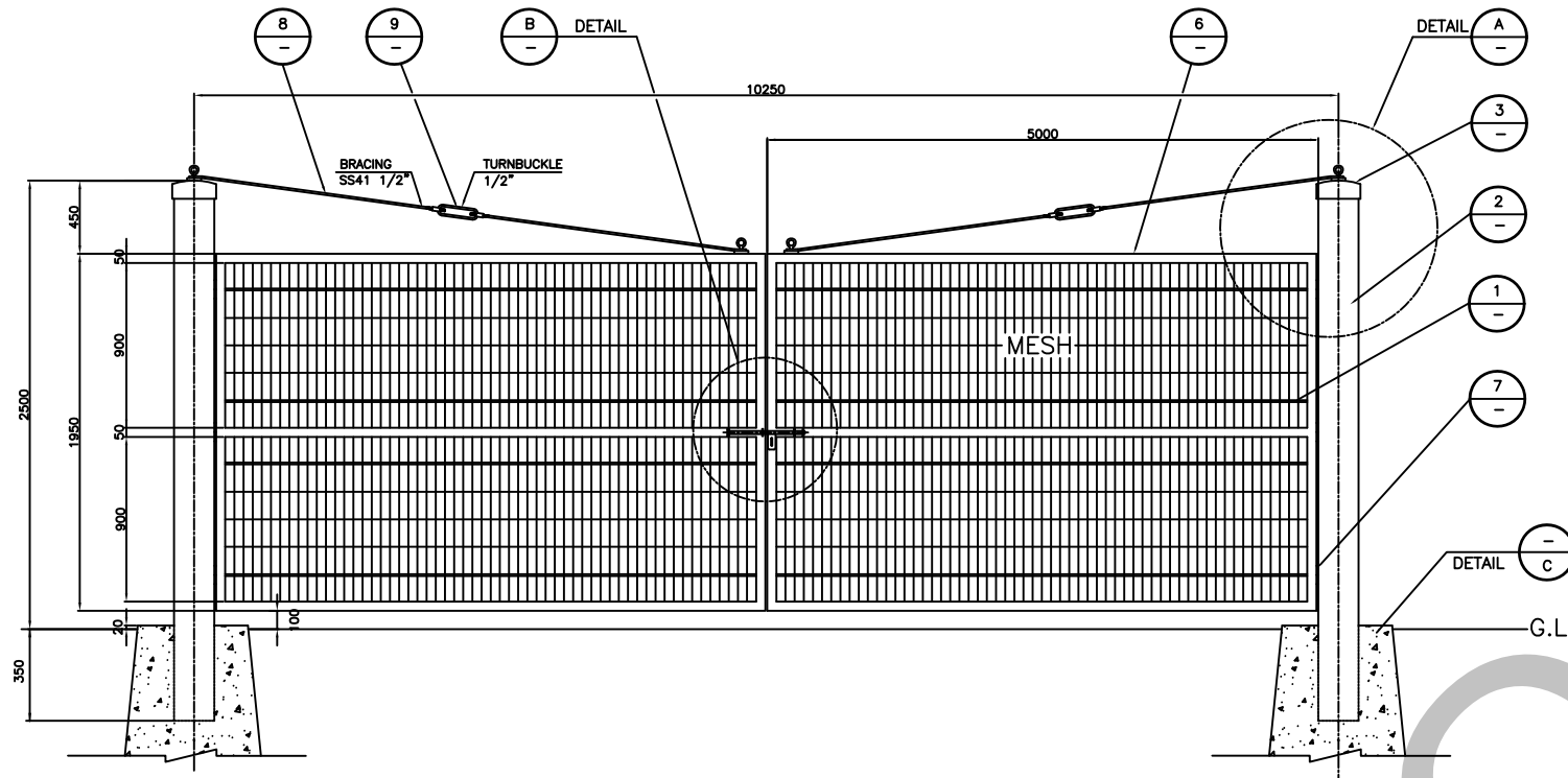
EXPTRIOR ELEVATION 001 AT WIRE MESH SWING GATE SCALE : 1 / NONE
